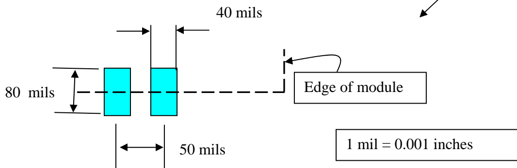
Figure 1-2 Top view of BT module mounting recommendations
